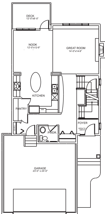
MAIN FLOOR PLAN ELEVATION MKI B
