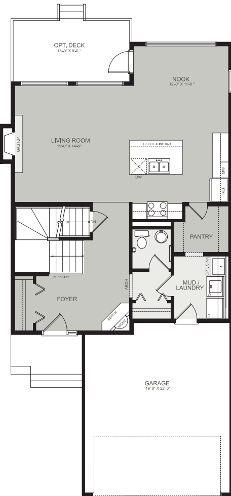
main 942 sq.ft
