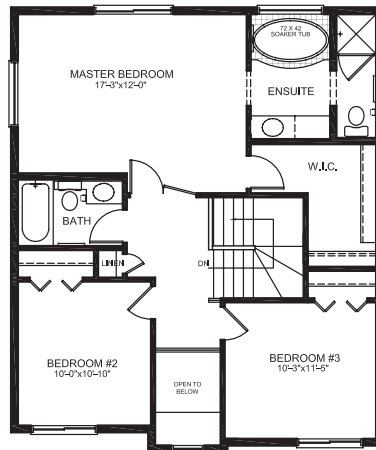
UPPER FLOOR PLAN 829 SQ. FT. 1790 TOTAL SQ. FT.
