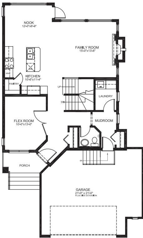
MAIN FLOOR PLAN 961 SQ. FT. 1790 TOTAL SQ. FT.
